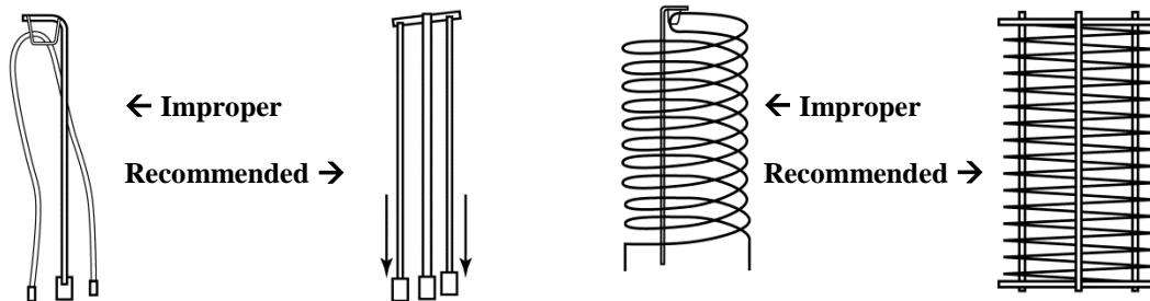
Figure 2. Supported and unsupported filaments and anode grids.
