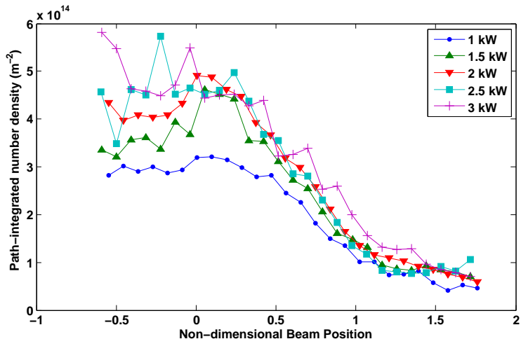
Figure 7. Path-integrated boron number densities as a function of channel position. The thruster was held at 500 V for each condition.
