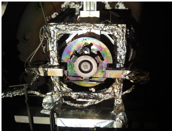
Figure 5. Picture of the HiVHAc thruster and CRDS setup within the VF8 chamber. The optical frame was wrapped in 3 layers of foil to help reduce misalignment induced by heating.
