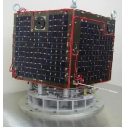
Fig. 1. Photo of 1st PROITERES satellite.
